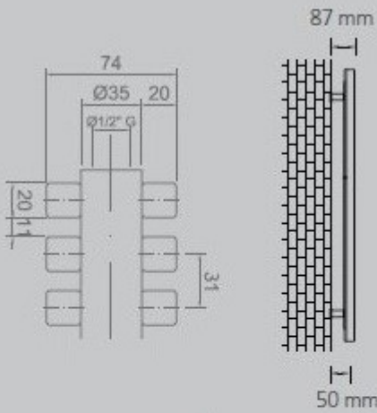
Filo muro - centro valvola Push to wall - valve center
